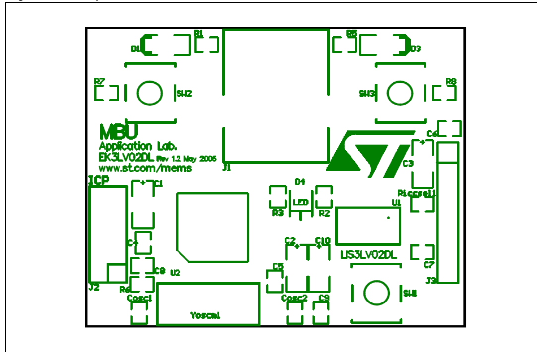
Figure 2. Top silk-screen for EK3LV02DL kit
