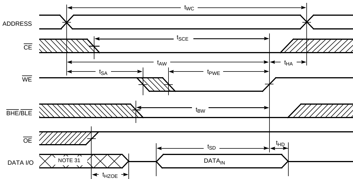
Figure 9. Write Cycle No. 2: \overline{\text{CE}} Controlled [27, 28, 29, 30]
