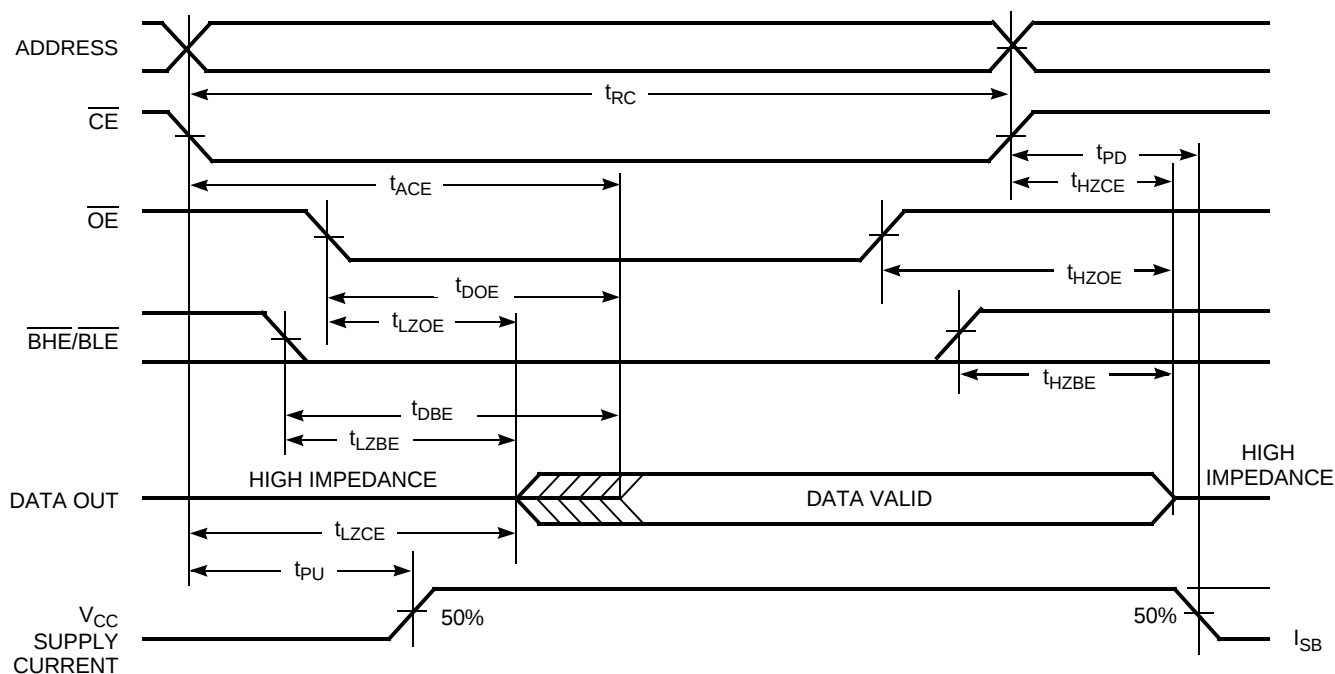
Figure 7. Read Cycle No. 2: \overline{\text{OE}} Controlled [24, 25, 26]
