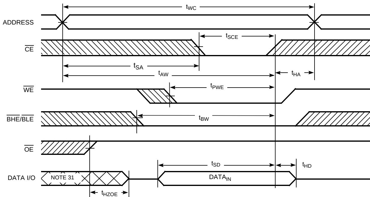
Figure 9. Write Cycle No. 2: \overline{\text{CE}} Controlled [27, 28, 29, 30]
