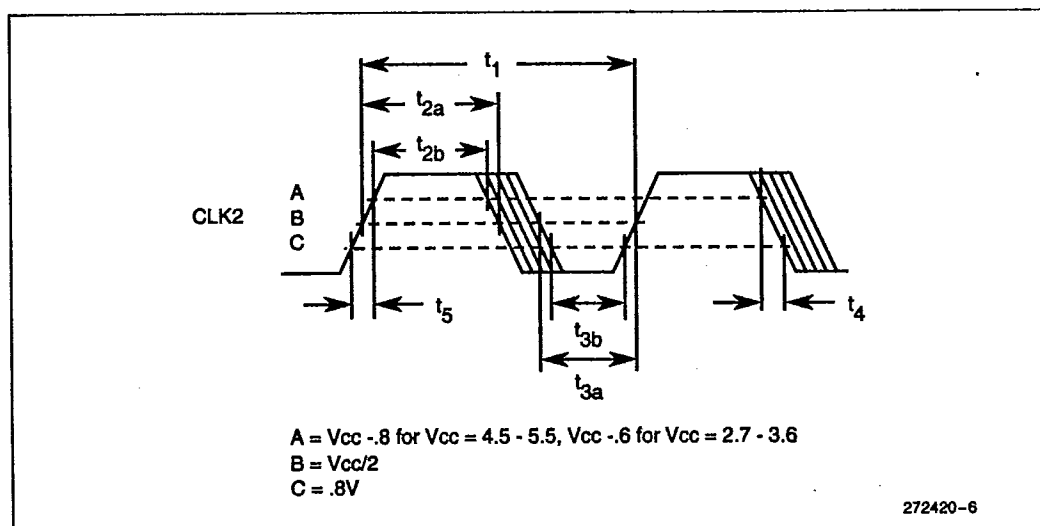
Figure 6. CLK2 Waveform
