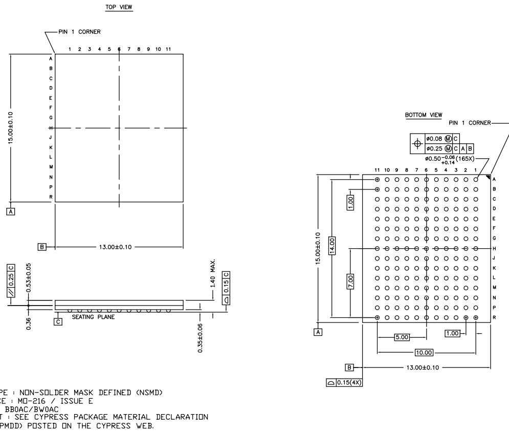
Figure 10. 165-ball FBGA (13 × 15 × 1.4 mm) BB165D/BW165D (0.5 Ball Diameter) Package Outline, 51-85180
