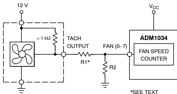
Figure 38. Fan with Strong TACH. Pullup to >V_{\text{CC}} or Totem-Pole Output, Attenuated with R1/R2
