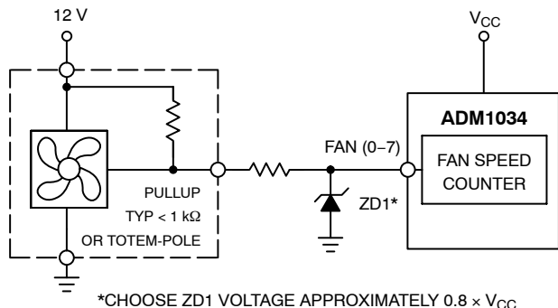
Figure 37. Fan with Strong TACH. Pullup to >V_{\text{CC}} or Totem-Pole Output, Clamped with Zener and Resistor
