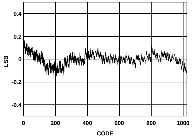
FIGURE 18. INTEGRAL NONLINEARITY
