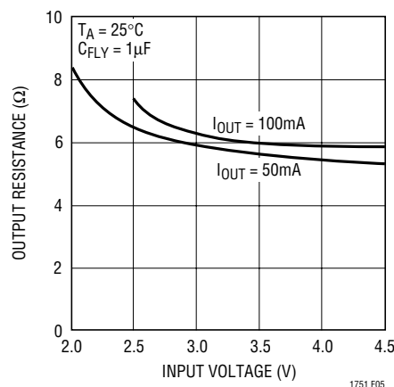
Figure 5. Typical R_{OUT} vs Input Voltage
