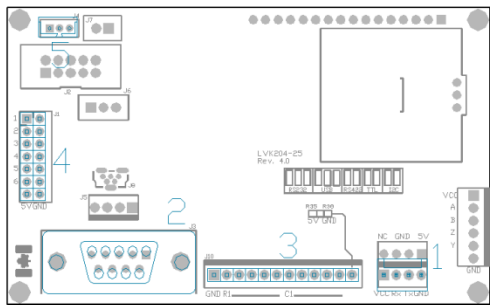
Figure 3: Standard Connections
