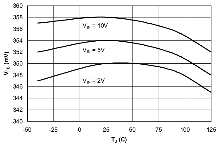
Average Feedback Voltage vs. Junction Temperature vs. Input Voltage
