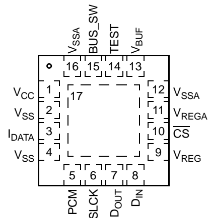
PIN CONNECTIONS
