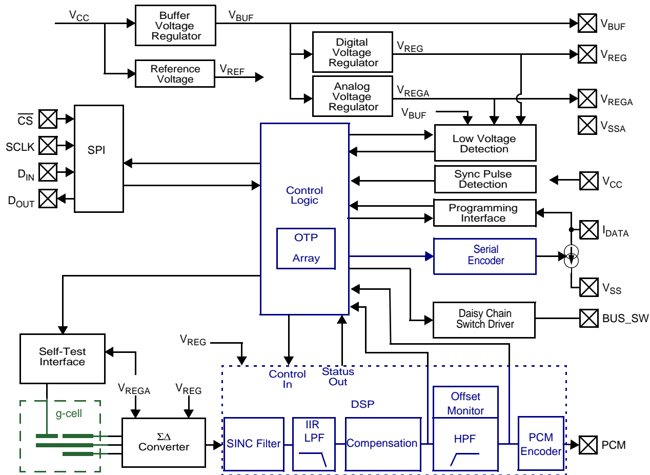
Figure 3. Block Diagram
