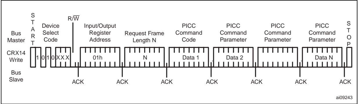
Figure 14. Host-to-CRX14 Transfer: I 2 C Write to Input/Output Frame Register for ISO14443B
