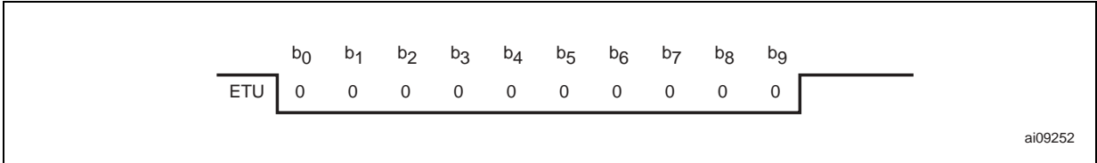
Figure 23. Request End Of Frame
