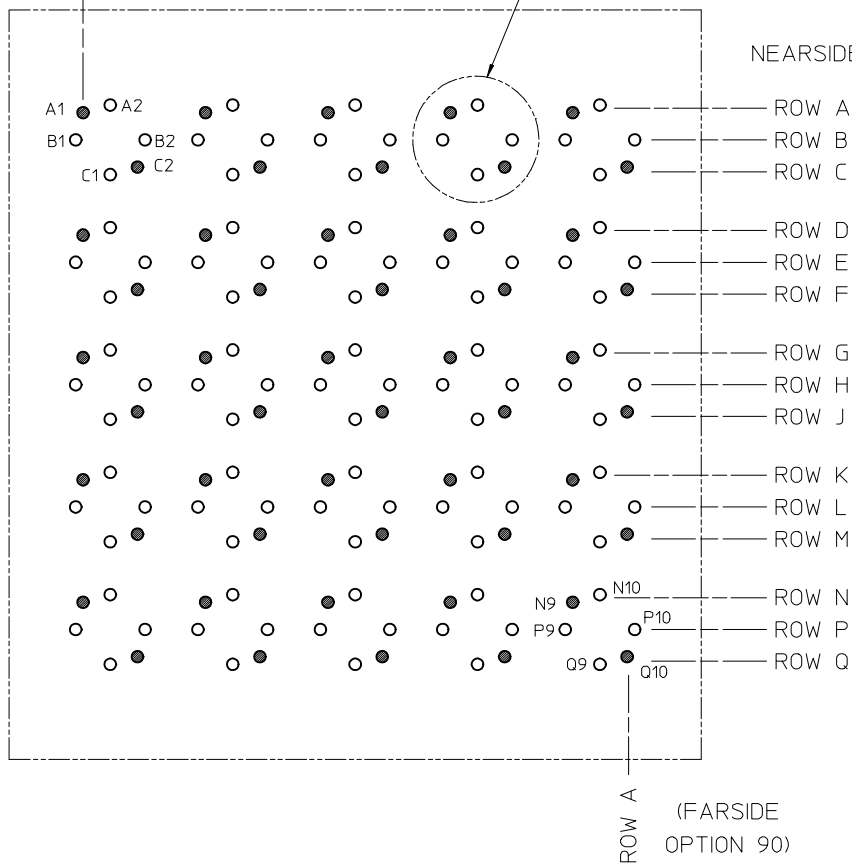
MIDPLANE PCB LAYOUT SCALE 8:1
