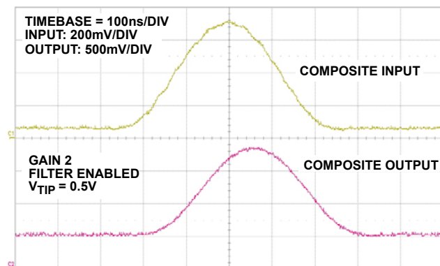
FIGURE 12. 2T RESPONSE
