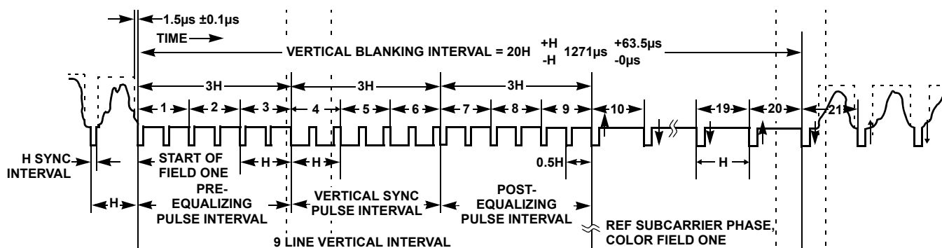
SIGNAL 1b. VERTICAL SYNC OUTPUT
