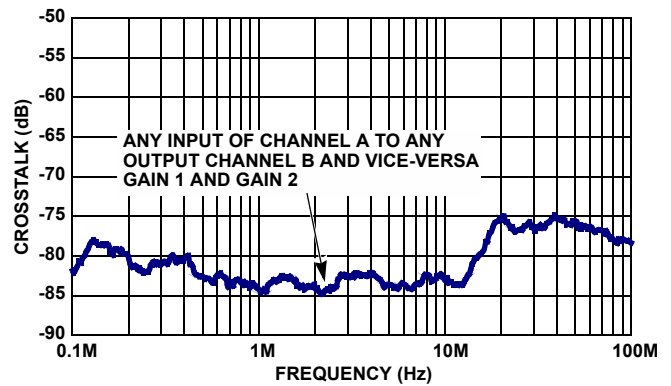
FIGURE 22. INTER-CHANNEL CROSSTALK
