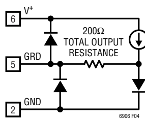
Figure 4. GRD Pin
