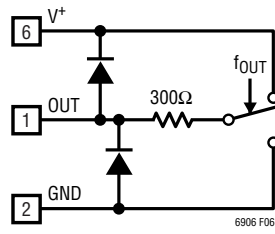
Figure 6. OUT Pin
