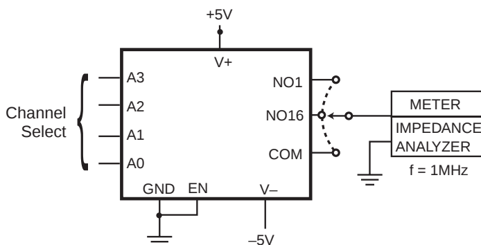
Figure 8. NO/COM Capacitance
