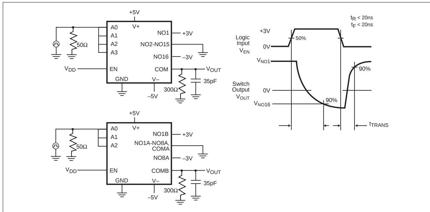
Figure 2. Transition Time
