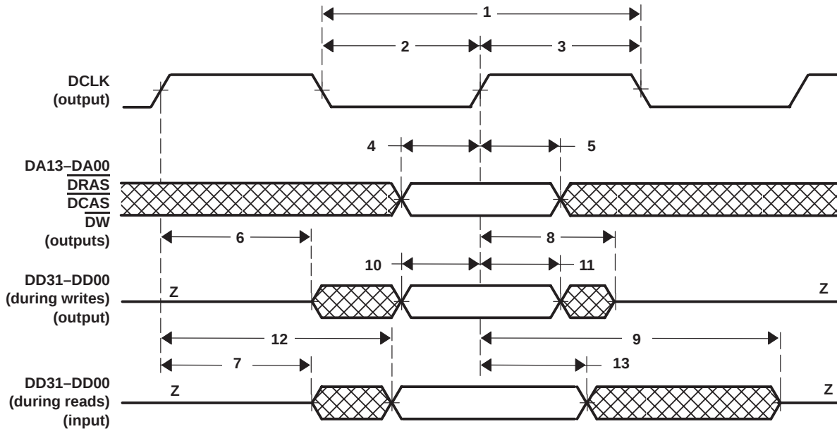
Figure 17. SDRAM Subcycle
