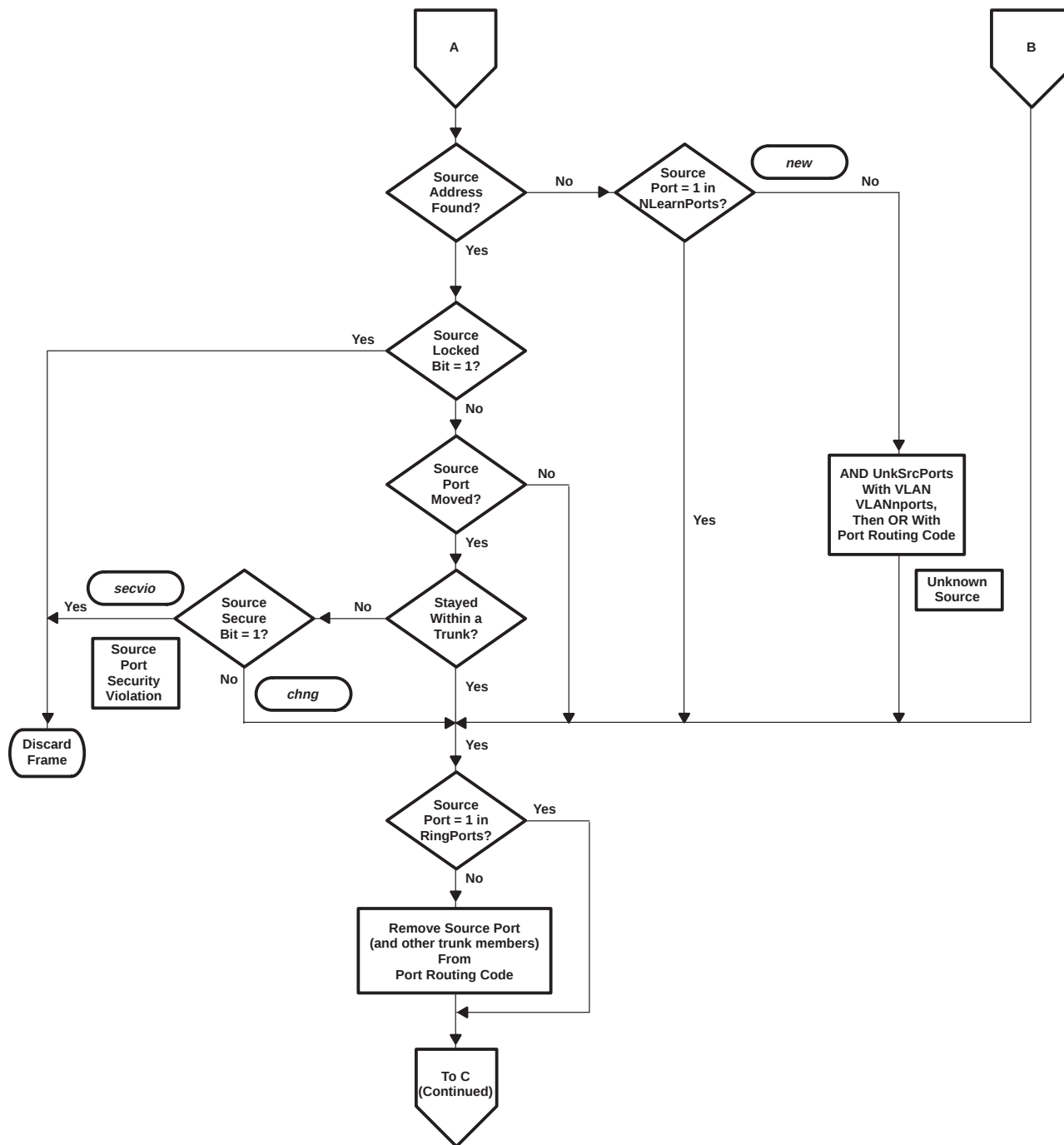
Figure 9. Frame-Routing Algorithm (Continued)
