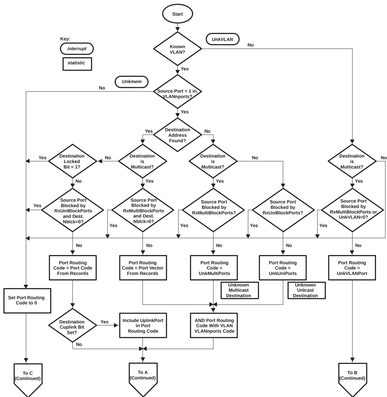
Figure 9. Frame-Routing Algorithm
