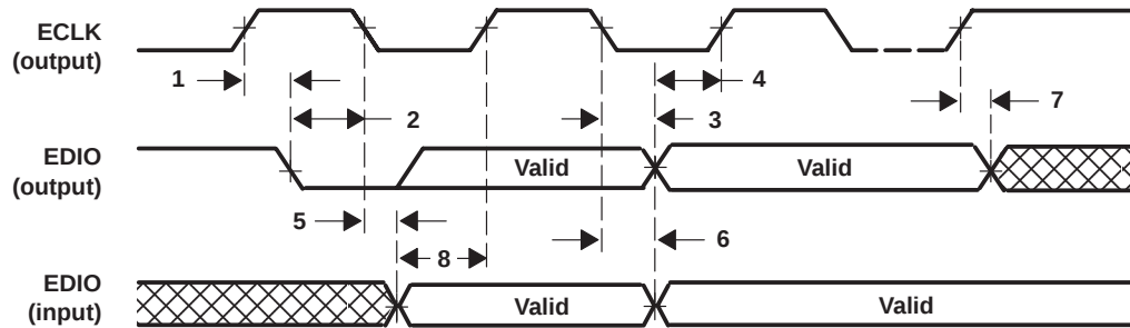
Figure 21. EEPROM
