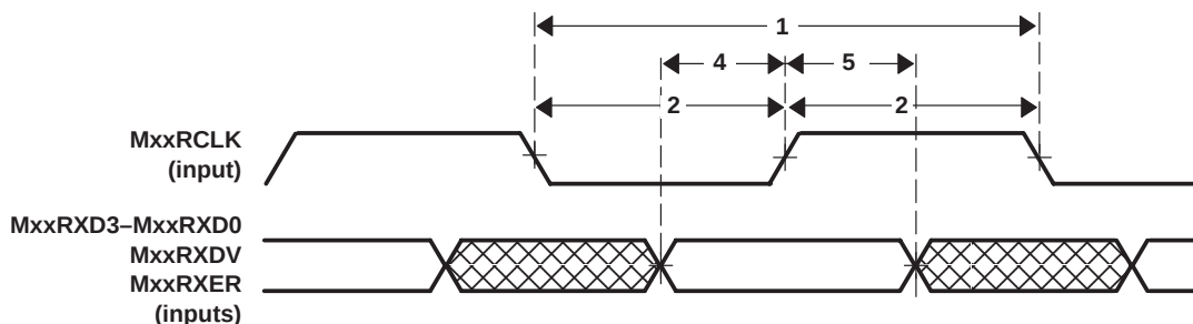
Figure 14. 10-/100-Mbit/s Receive Ports
