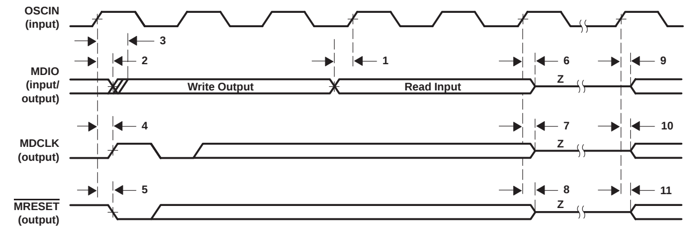
Figure 20. Serial MII Management Read/Write Cycle
