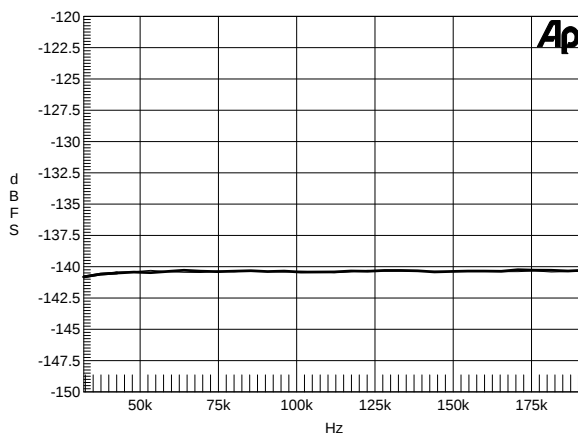
-60 dBFS 1 kHz Tone, Fsi = 96 kHz
