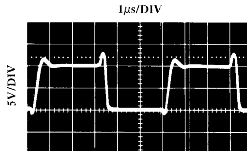
Figure 24. Output Waveform
