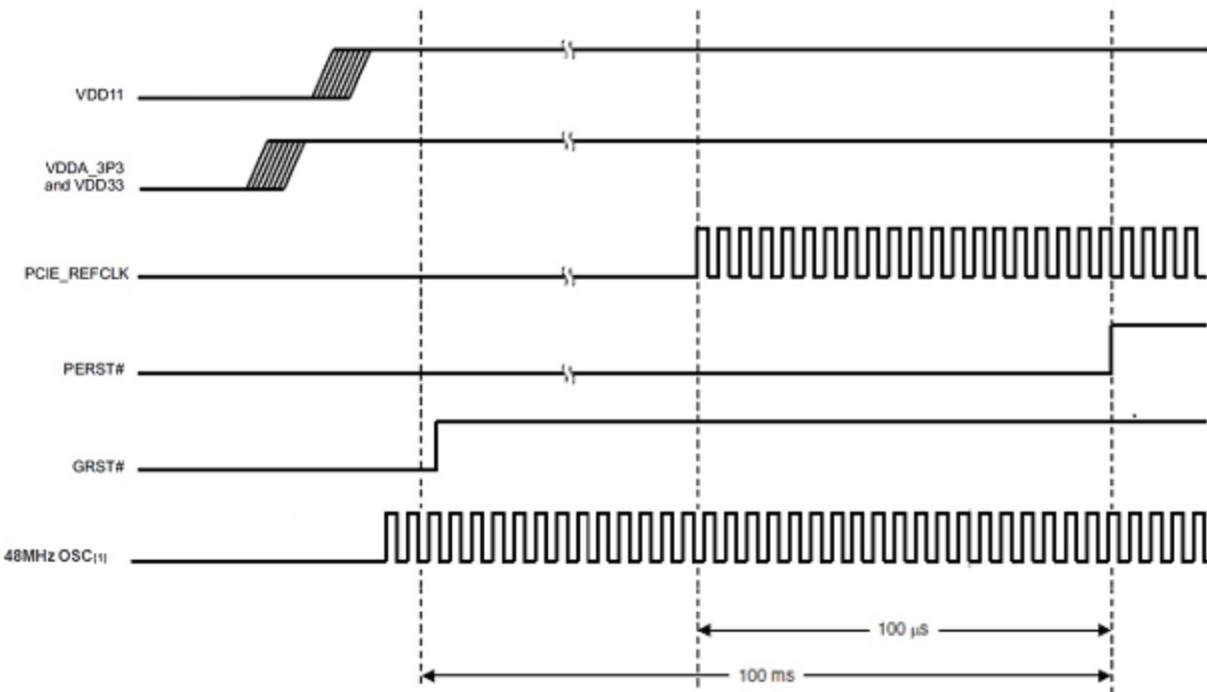
Figure 7-16. Power-Up Sequence
