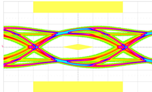
Figure 7-11. Super-Speed Downstream Port 4
