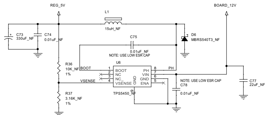
Figure 7-7. Reference Design 5
