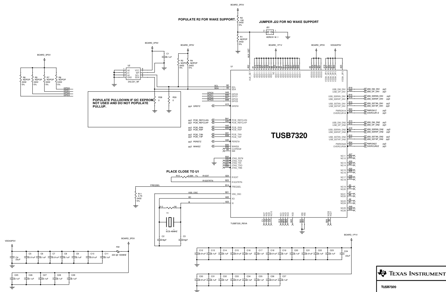
Figure 7-3. Reference Design 1
