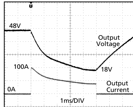
Fig. 25-4 Peak load 100A for 5ms, typ.
