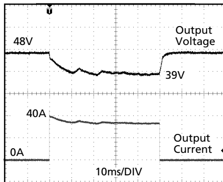
Fig. 25-3 Peak load 40A for 50ms, typ.
