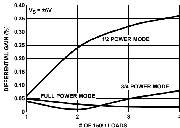
FIGURE 26. DIFFERENTIAL GAIN
