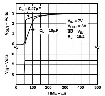
Figure 10. Power-Up Response
