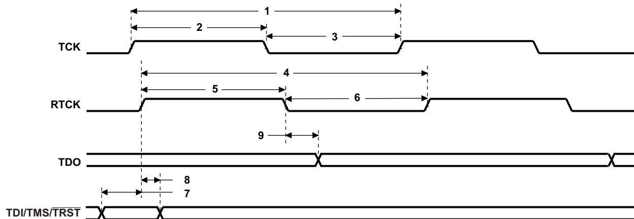
Figure 6-91. JTAG Test-Port Timing
