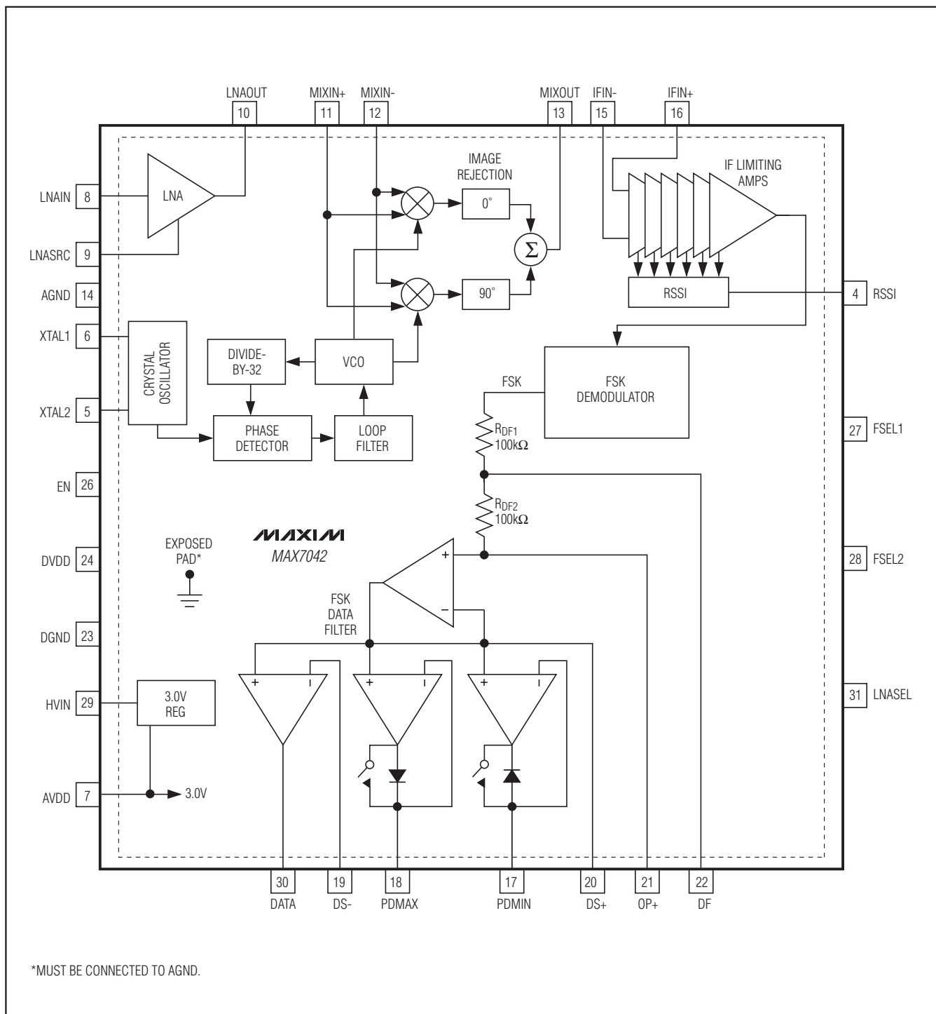
Functional Diagram
