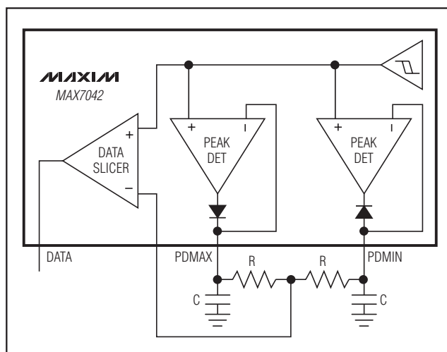
Figure 4. Generating Data-Slicer Threshold Using the Peak Detectors
