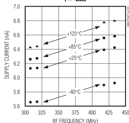
SUPPLY CURRENT vs. RF FREQUENCY (1x I_{LNA} )
