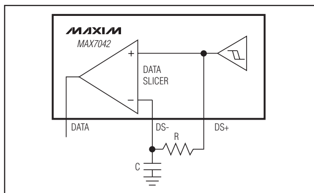
Figure 3. Generating Data-Slicer Threshold
