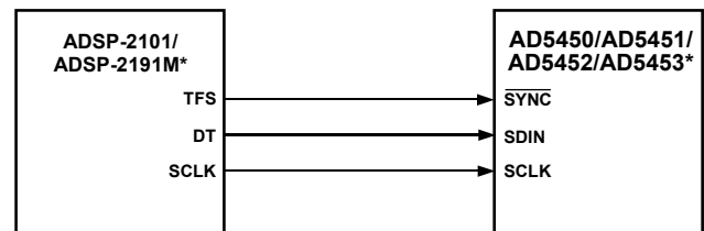
Figure 57. ADSP-2101/ADSP-2191M-to-AD5450/AD5451/AD5452/AD5453 Interface
