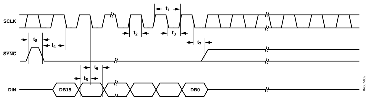
Figure 2. Timing Diagram
