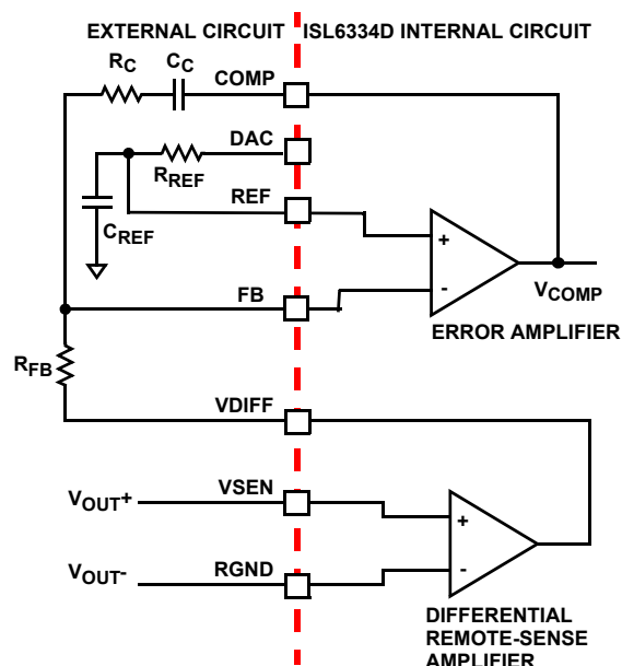
FIGURE 9. OUTPUT VOLTAGE REGULATION LOOP
