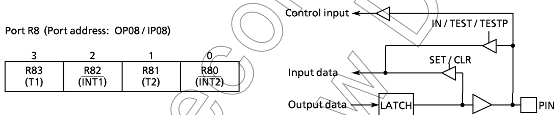
Figure 3-5. Port R8
