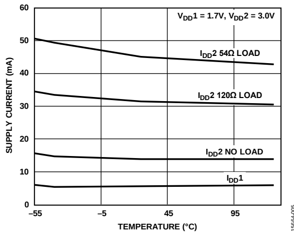
Figure 5. Supply Current ( I_C ) vs. Temperature at R_L = 54\ \Omega , 120\ \Omega , and No Load; Data Rate = 2.5 Mbps, V_{DD1} = 1.7\text{ V} , V_{DD2} = 3.0\text{ V}
