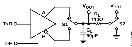
Figure 30. Driver Enable/Disable
