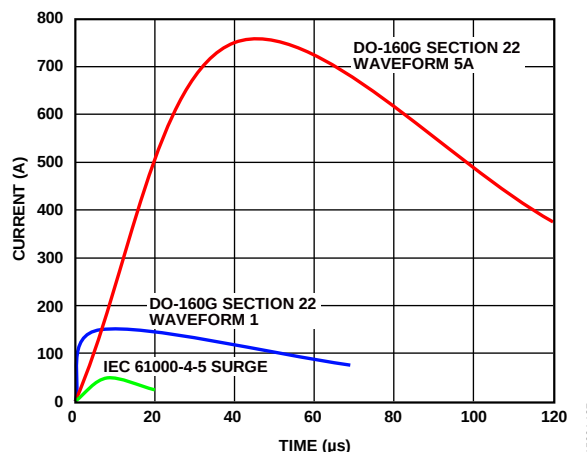
Figure 37. DO-160G Section 22 Waveform 1 and Waveform 5A, and IEC61000-4-5 Surge Waveform
