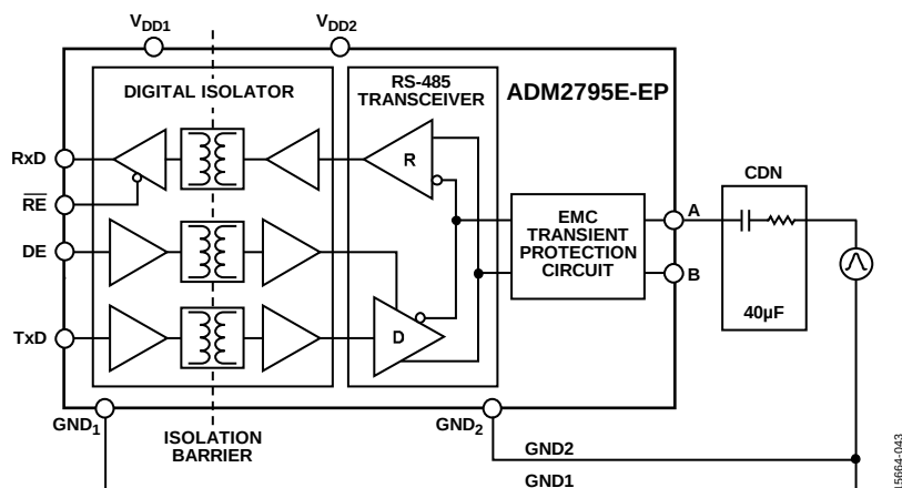
Figure 38. DO-160G Section 22 Waveform 3 Test Setup CDN
