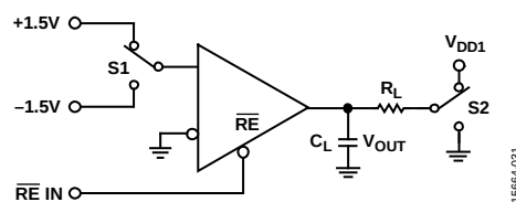
Figure 32. Receiver Enable/Disable
