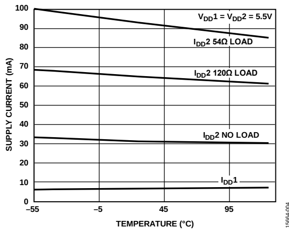
Figure 4. Supply Current ( I_C ) vs. Temperature at R_L = 54\ \Omega , 120\ \Omega , and No Load; Data Rate = 2.5 Mbps, V_{DD1} = 5.5\text{ V} , V_{DD2} = 5.5\text{ V}
