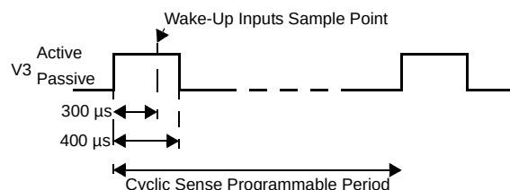
Figure 10. V3 Timing
