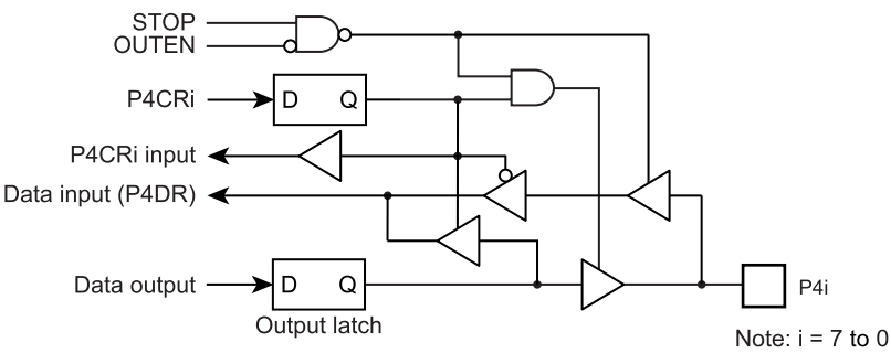
Figure 7-6 Port P4
