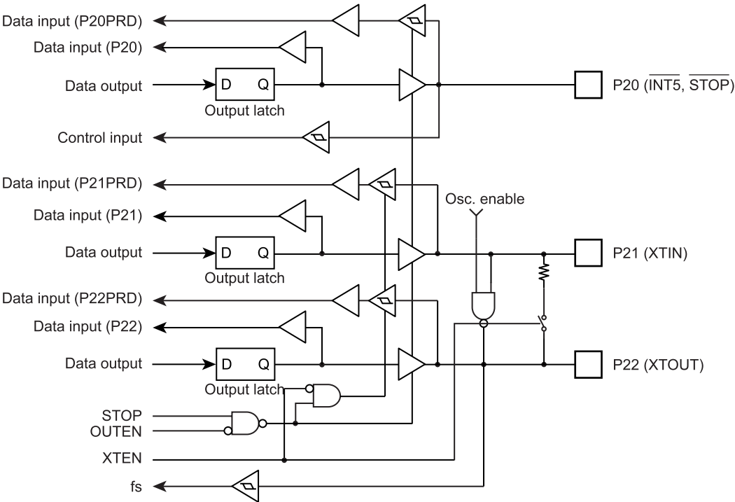
Figure 7-4 Port P2
