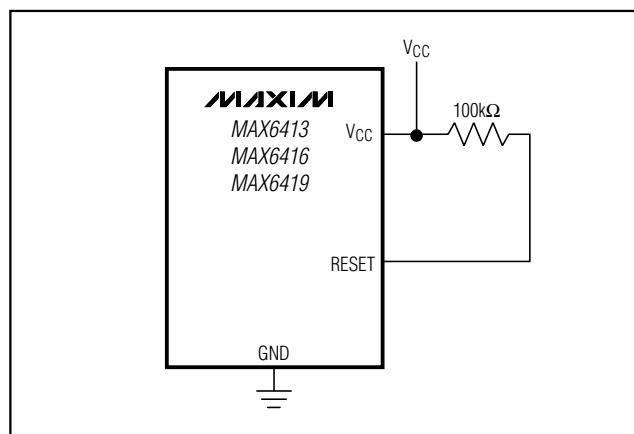
Figure 7. Ensuring \overline{\text{RESET}} Valid to V_{CC} = 0
