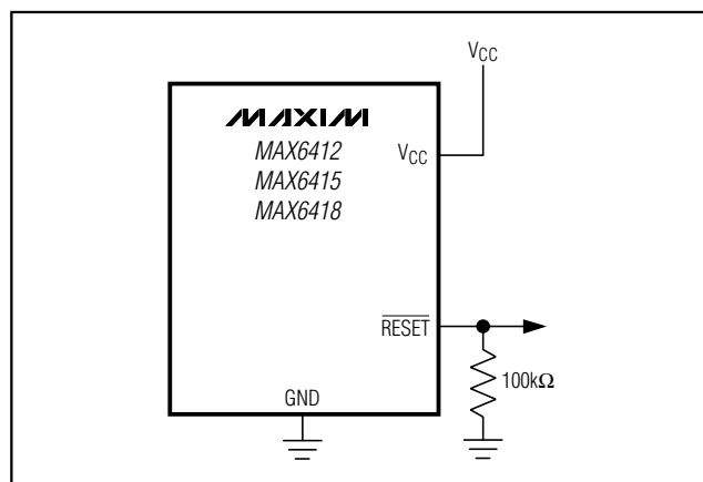
Figure 6. Ensuring \overline{\text{RESET}} Valid to V_{CC} = 0
