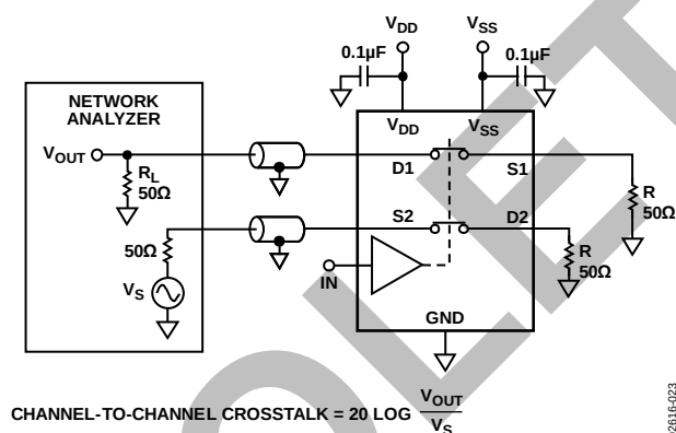
Figure 23. Channel-to-Channel Crosstalk
