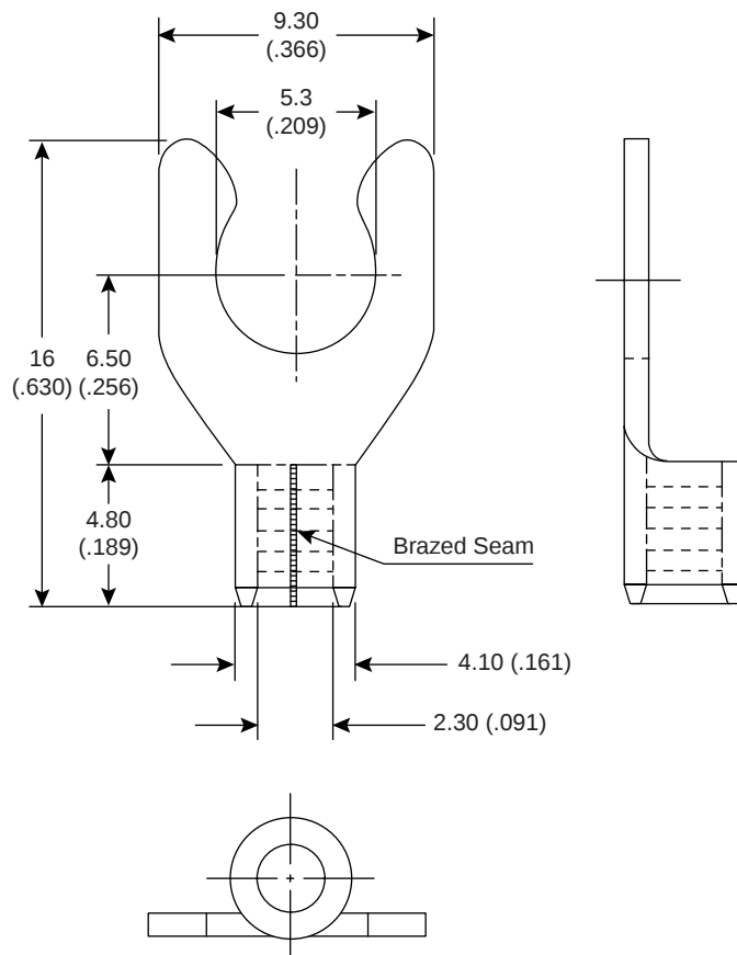
Dimensions mm (In.)
