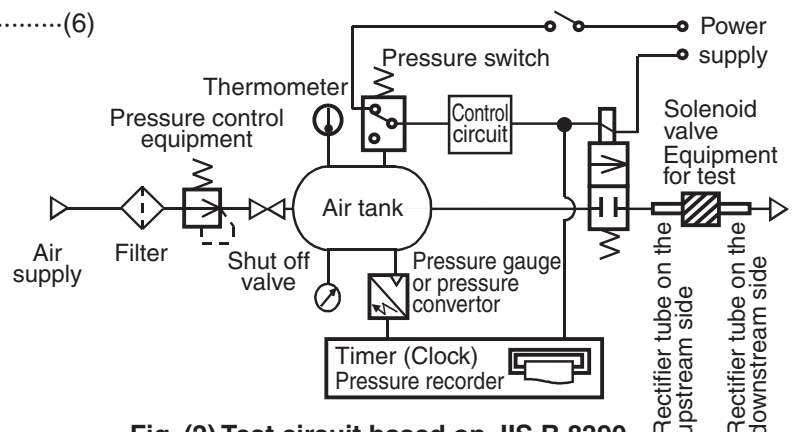
Fig. (2) Test circuit based on JIS B 8390
