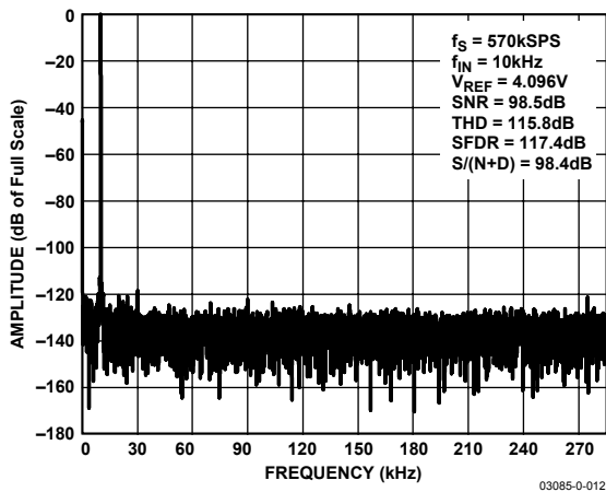
Figure 12. FFT (10 kHz Tone)
