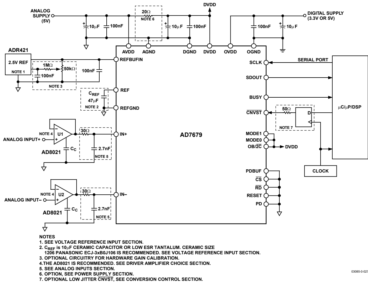
Figure 25. Typical Connection Diagram (Internal Reference Buffer, Serial Interface)
