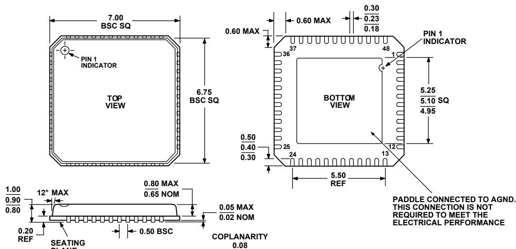
Figure 45. 48-Lead Frame Chip Scale Package [LFCSP] (CP-48) (Dimensions shown in millimeters)
