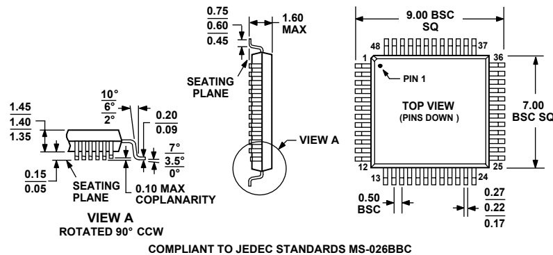
Figure 44. 48-Lead Quad Flatpack [LQFP] (ST-48) (Dimensions shown in millimeters)
