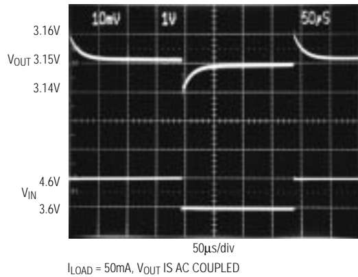
LINE TRANSIENT
