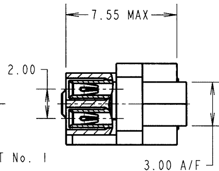
PART SECTION X-X
