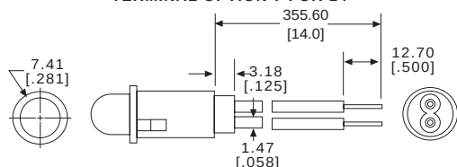
24 AWG WIRE LEADS - TERMINAL OPTION 3 FOR 6" WIRE LEADS TERMINAL OPTION 7 FOR 14" WIRE LEADS
