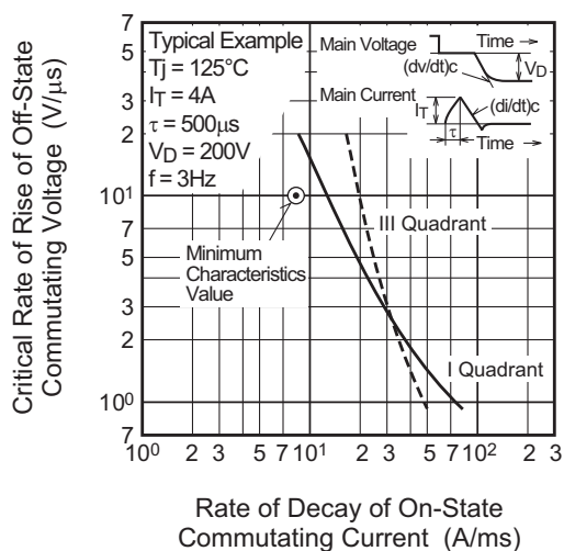
Commutation Characteristics
