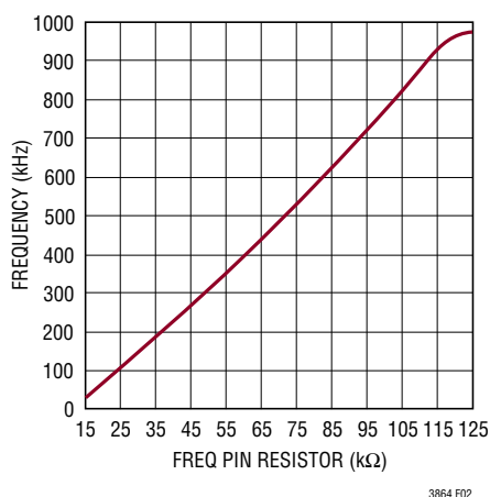
Figure 2. Switching Frequency vs Resistor on FREQ
