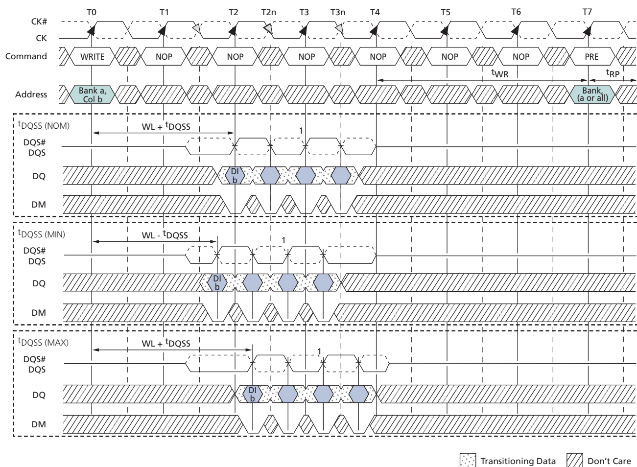
Figure 61: WRITE-to-PRECHARGE
