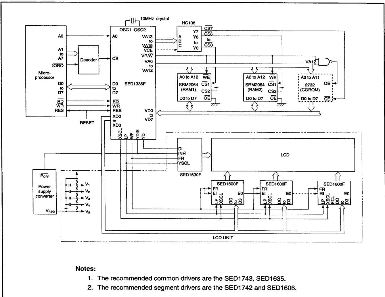
Figure 86. System interconnection diagram
