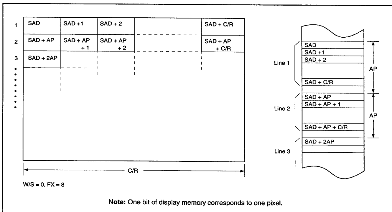
Figure 50. Character parameters vs. memory
