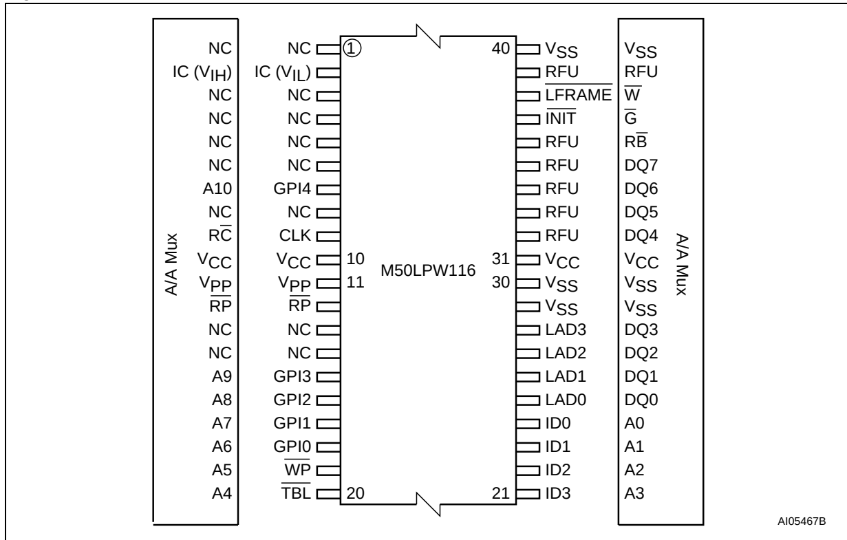
Figure 4. TSOP Connections
