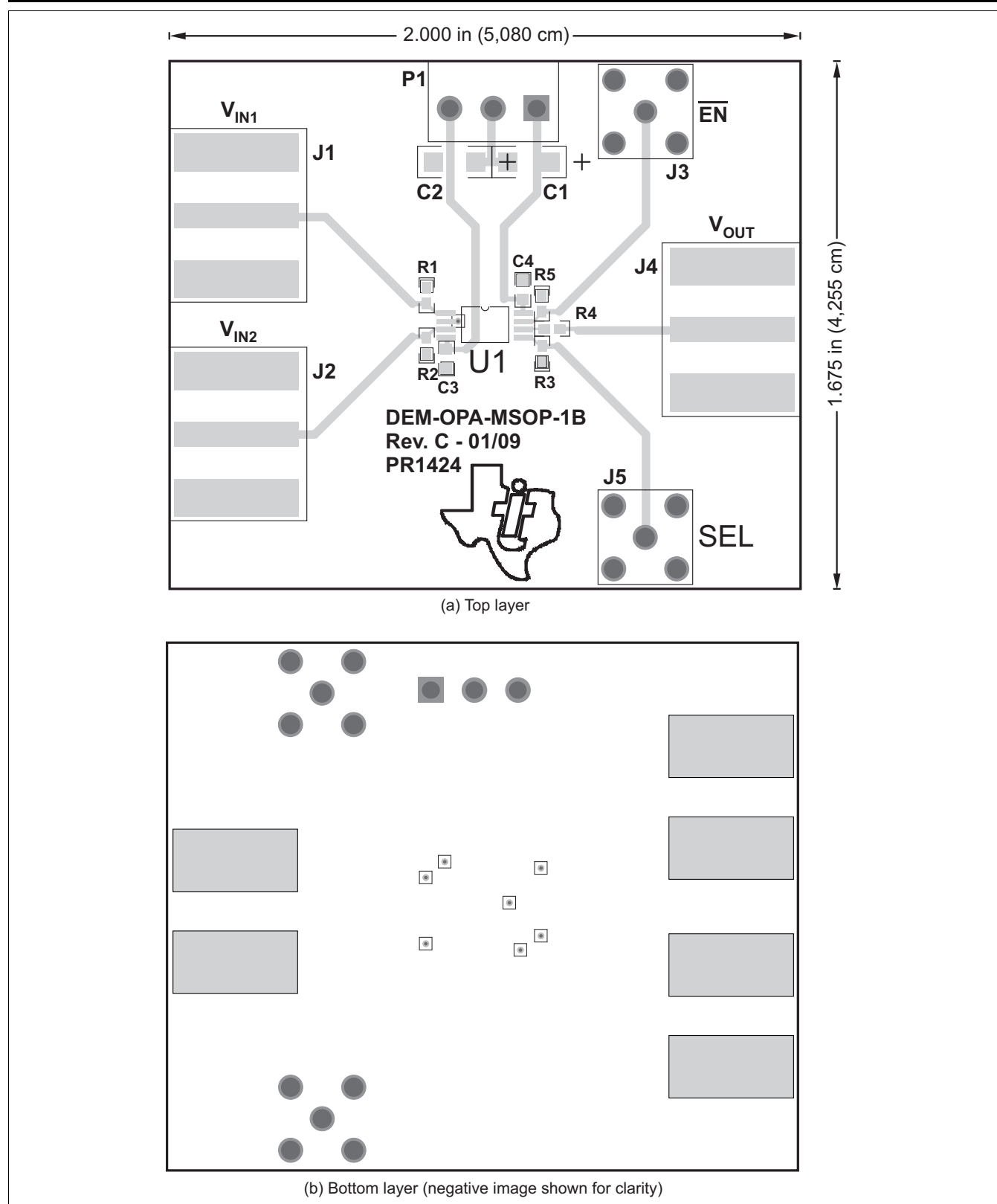
Figure 3. DEM-OPA-MSOP-1B Demonstration Fixture Layout
