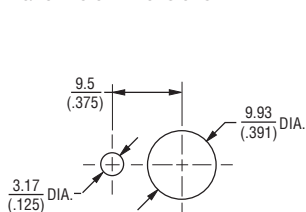
Panel Hole Dimensions
