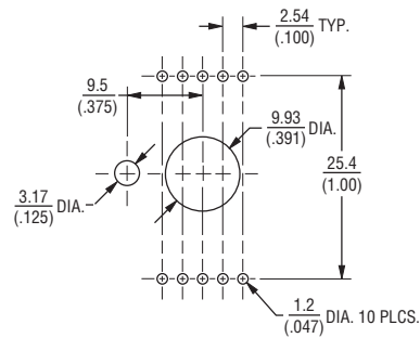
PCB Board Hole Pattern w/PCB Bracket
