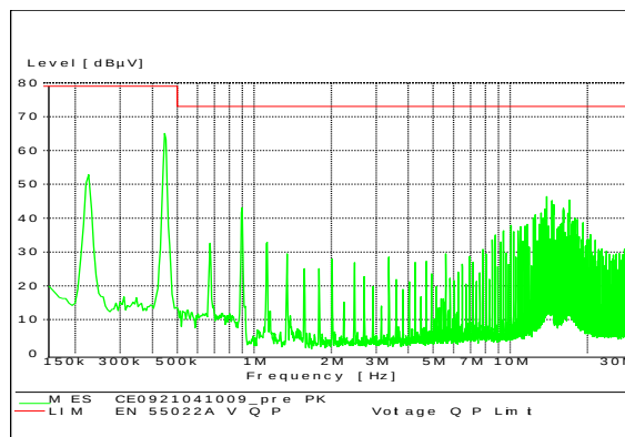
Figure 44. KW015A0F Quasi Peak Conducted Emissions with EN 55022 Class A limits, no external filter ( V_{IN} = V_{IN,NOM} , I_o = 0.85 I_{o,max} ).
