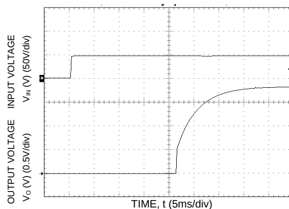
Figure 24. Typical Start-up Using Input Voltage ( V_{IN} = V_{IN,NOM} , I_o = I_{o,max} ).
