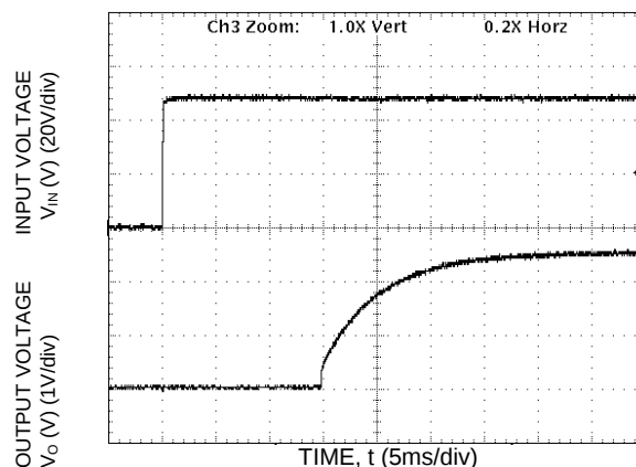
Figure 18. Typical Start-up Using Input Voltage ( V_{IN} = V_{IN,NOM} , I_o = I_{o,max} ).
