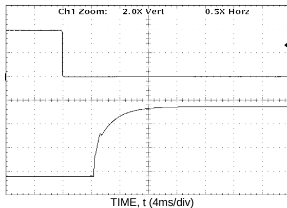
Figure 29. Typical Start-up Using Remote On/Off, negative logic version shown ( V_{IN} = V_{IN,NOM} , I_o = I_{o,max} ).
