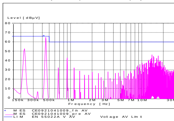
Figure 45. KW015A0F Average Conducted Emissions with EN 55022 Class A limits, no external filter ( V_{IN} = V_{IN,NOM} , I_o = 0.85 I_{o,max} ).
