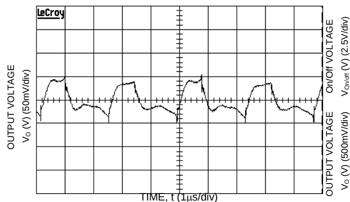
Figure 26. Typical output ripple and noise ( V_{IN} = V_{IN,NOM} , I_o = I_{o,max} ).
