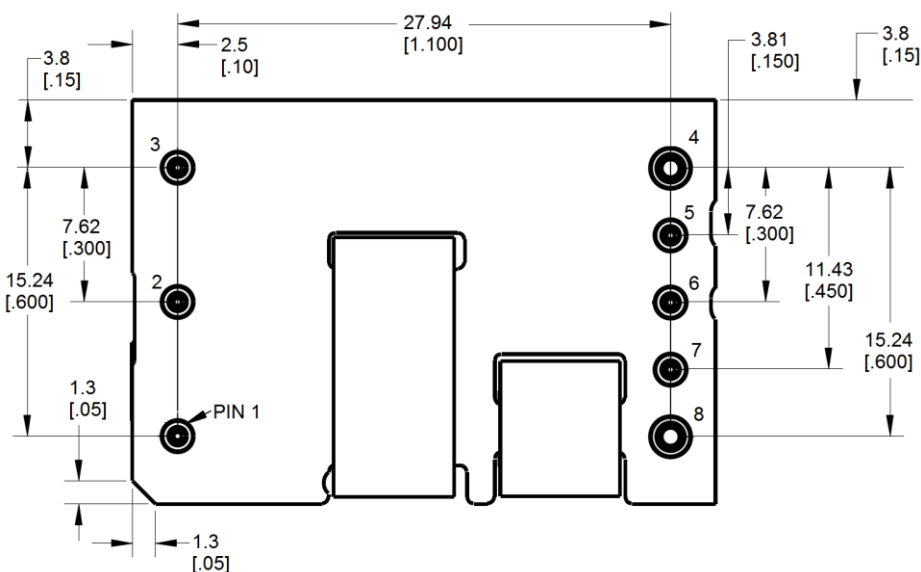
Bottom View
