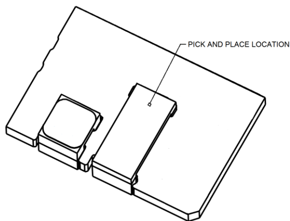
Figure 46. Pick and Place Location.
