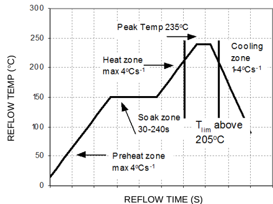
Figure 47. Reflow Profile for Tin/Lead (Sn/Pb) process
