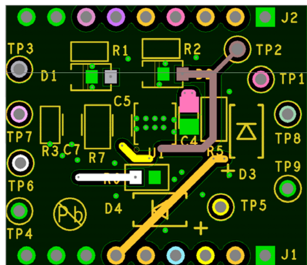
Figure 12. HIP2105DBEVAL1Z Bottom Layer
