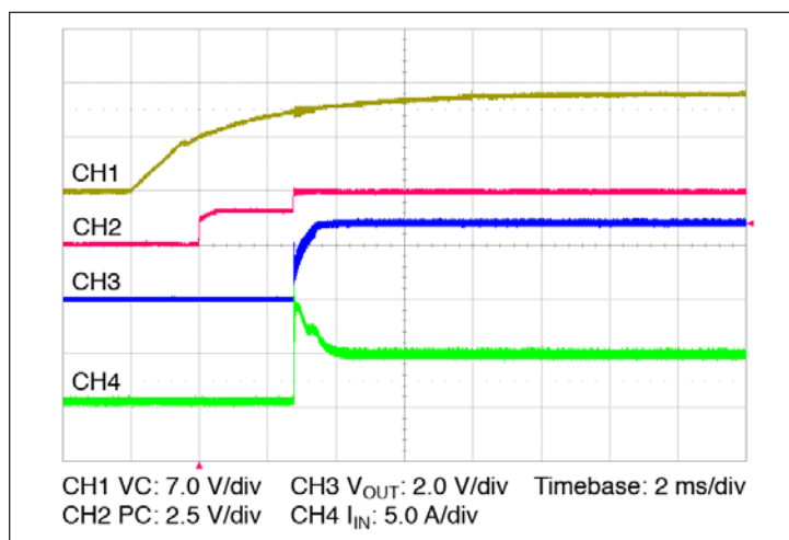
Figure 11 — Start up from application of VC; V_{IN} pre-applied C_{OUT} = 16000 \mu F
