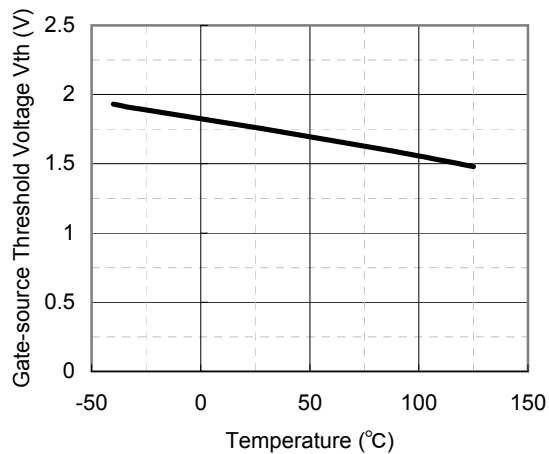
V th - T a
