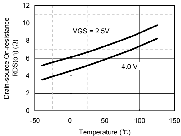
R DS(on) - T a
