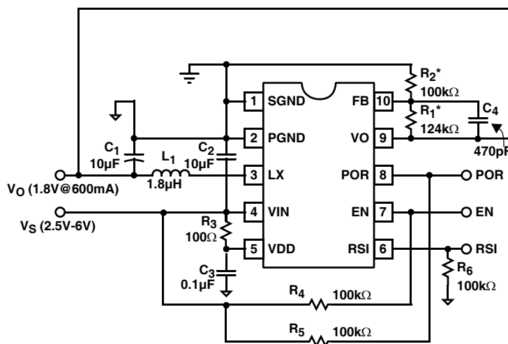
ISL97536 (10 LD MSOP) TOP VIEW
